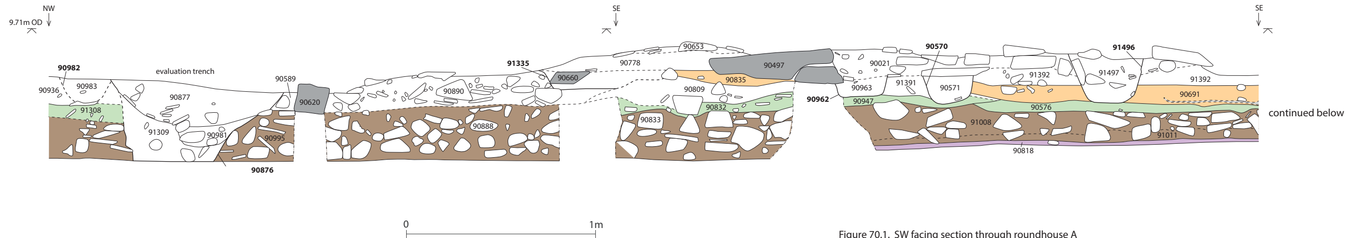
Figure 70.1. SW facing section through roundhouse A
