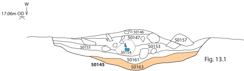
Figure 13. Sections of fire pits in the Neolithic building
