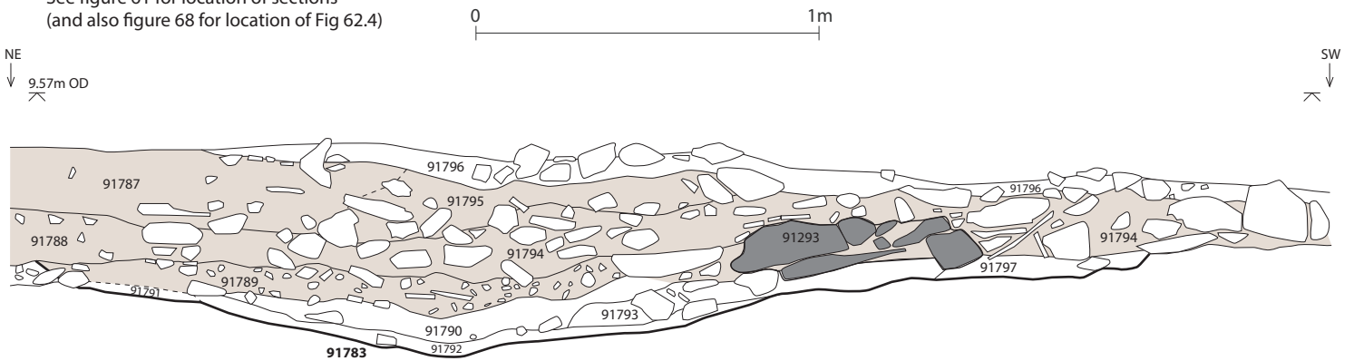
Fig 62.4. South-east facing section at an angle through ditch 91783 showing it sealed under later deposits
