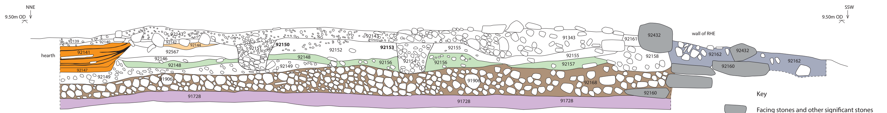
Figure 69.2. WNW facing section of SW quadrant of roundhouse E
