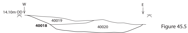
Figure 45. Sections across ring ditch
