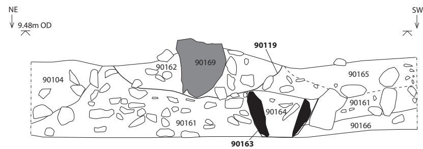
Figure 119.3. North-west facing section through wall 90169 and drain 90163
