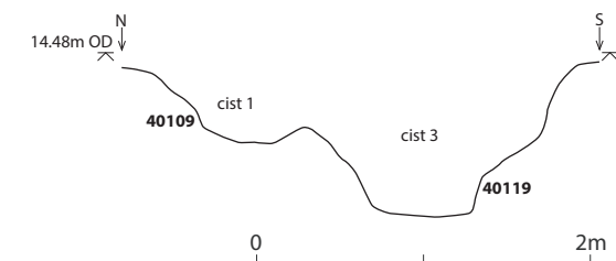
Figure 40.5 Profile through cists 1 and 3
