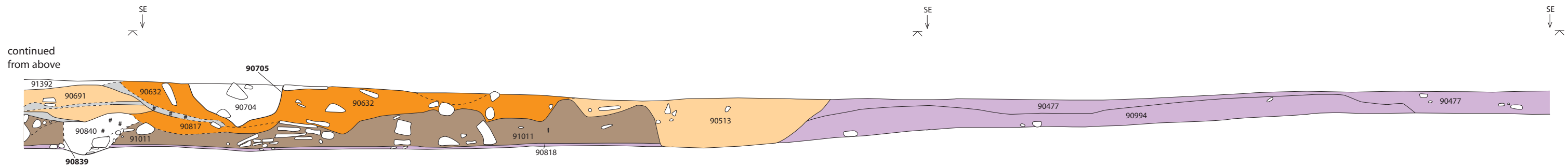
Figure 70.1. SW facing section through roundhouse A
