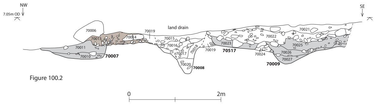
Figure 100. Sections of western end of trackway in Area J
