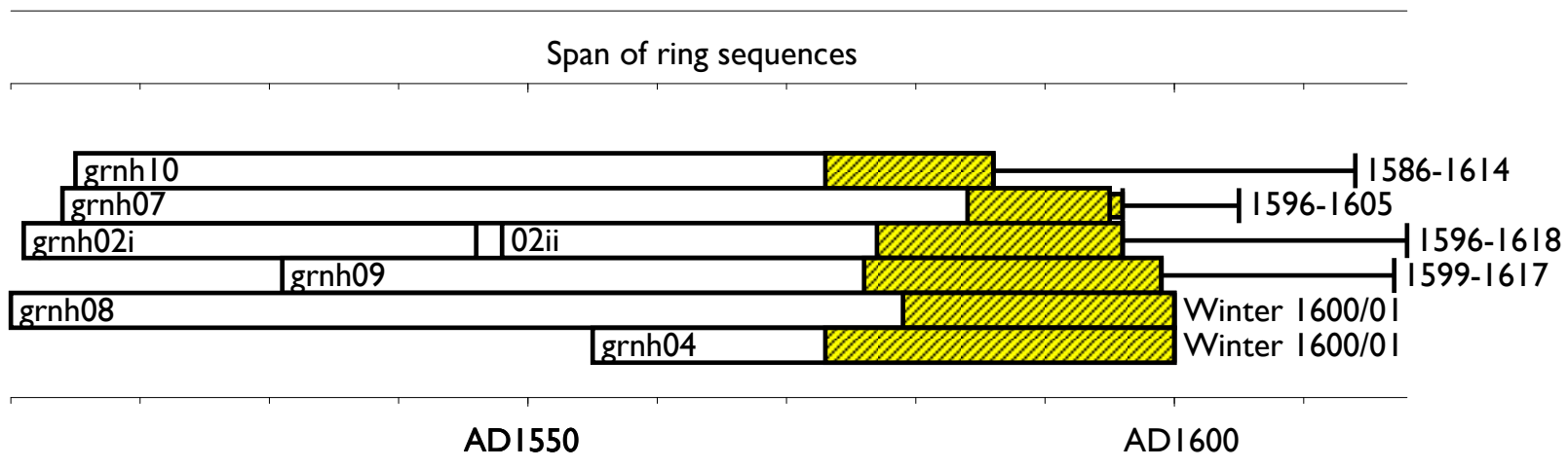
Figure 3: Bar diagram showing the relative positions of overlap of the dated samples, with their actual or likely felling dates / date ranges. White sections represent heartwood rings and yellow hatched sections represent sapwood, narrow bars represent additional unmeasured rings.
