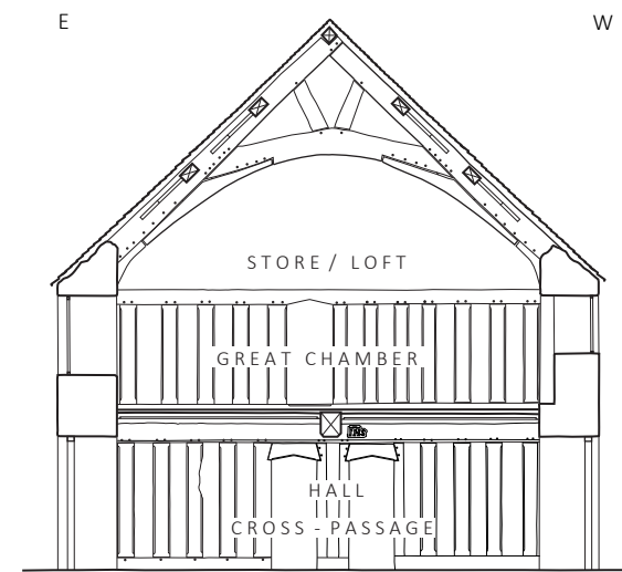
(c) Transverse section
