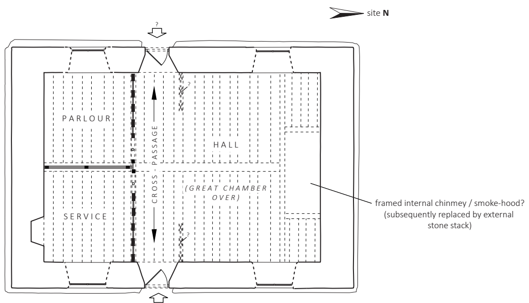
(a) Ground floor plan
